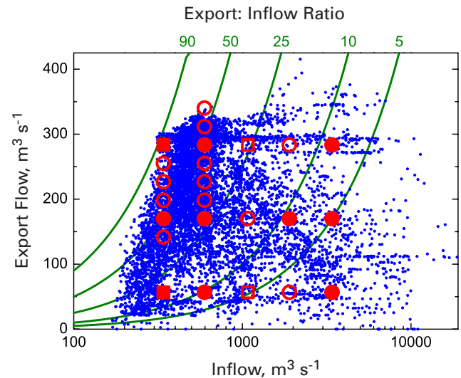
Figure 2. Daily export flow and inflow from the Dayflow accounting program for 1980–2002 (blue symbols) and values used in the model (red). Open symbols are base run only, filled symbols are other runs as described in Table 3. Squares are combinations used in examples (Figures 5 and 6). Green lines give isopleths of export:inflow (EI) ratio.
